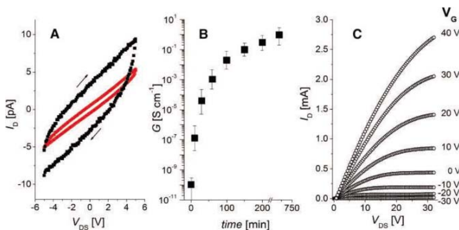
Fig. 2. (A) I - V scans for a film of 8-nm oleic acid capped PbSe nanocrystals in which the voltage scan rate is 0.5 \text{V s}^{-1} (black) and 0.025 \text{V s}^{-1} (red) and the channel length L and width W are 6 \mu\text{m} and 5000 \mu\text{m} , respectively. (B) Conductance G of a PbSe nanocrystal film versus time of exposure to a 1 M solution of \text{N}_2\text{H}_4 in acetonitrile. The error bars show the spread in data from five samples. (C) Plot of drain current I_D versus drain-source voltage V_{DS} , as a function of V_G for a nanocrystal FET with a channel composed of 8-nm PbSe nanocrystals treated with hydrazine solution for 12 hours ( L = 10 \mu\text{m} , W = 2000 \mu\text{m} , with a 100-nm-thick \text{SiO}_2 gate dielectric).
